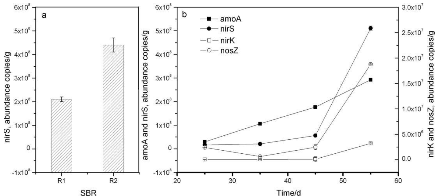
Fig 6. Absolute abundance of functional genes. (a) nirS abundance in two parallel SBRs on 46d; (b) amoA , nirK , nirS and nosZ abundance in the bioaugmented SBR. Error bars indicate standard deviations of three replicates. Invisible error bars indicate that standard deviations are smaller than the marker size.
