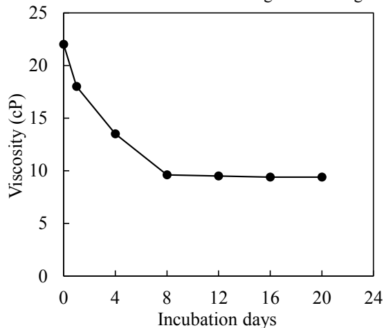
Fig. 4. Viscosity reduction of waxy crude oil throughout the degradation.
