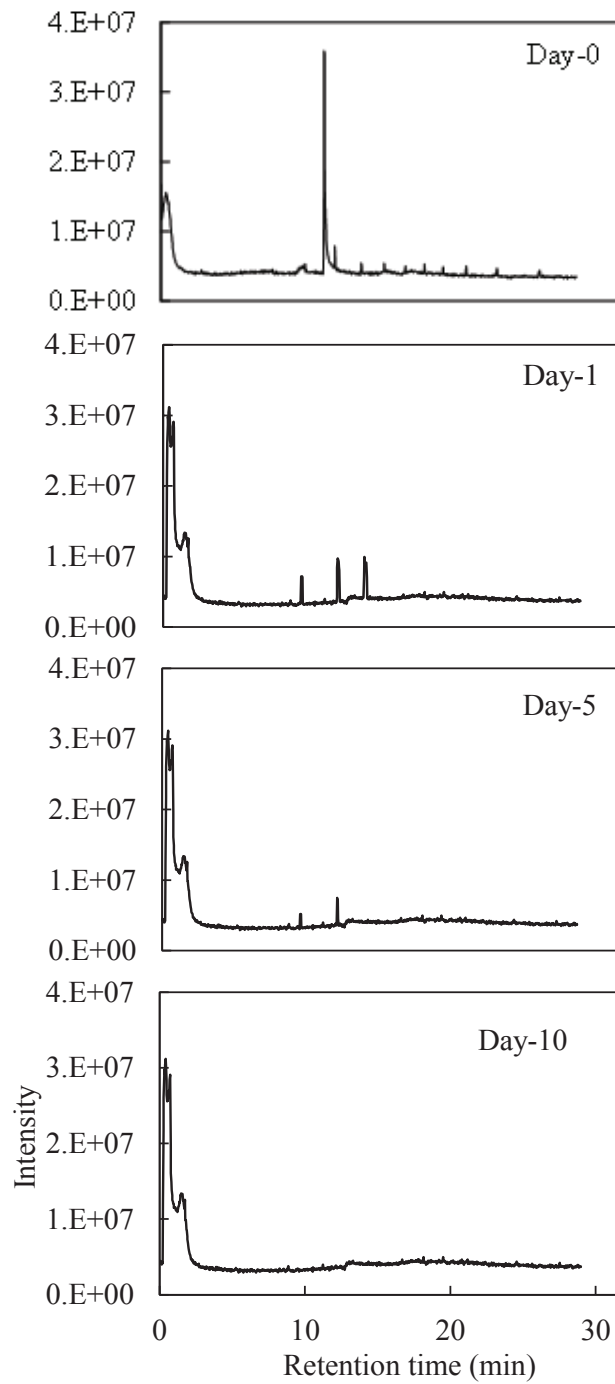
Fig. 5. Gas chromatograms before and after degradation of waxy crude oil using Bacillus subtilis .
