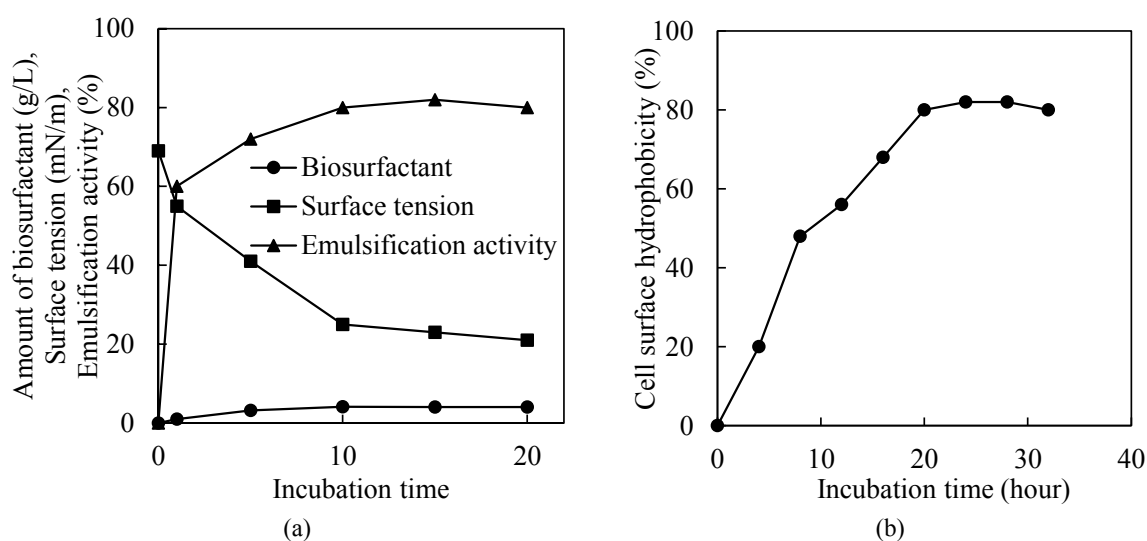
Fig. 3. (a) Production and properties of biosurfactant; (b) Bacterial adherence to waxy crude oil.
