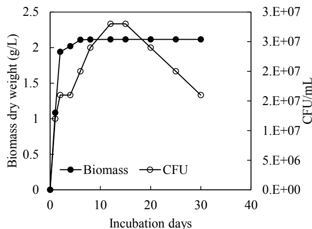
Fig. 2. Growth of Bacillus subtilis on waxy crude oil
